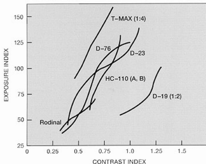
Toe speed of Kodak T-Max 100 vs. contrast index in various developers. My plot of Judge and Holm's data, previously published in Kodak Tech Bits 1991.
